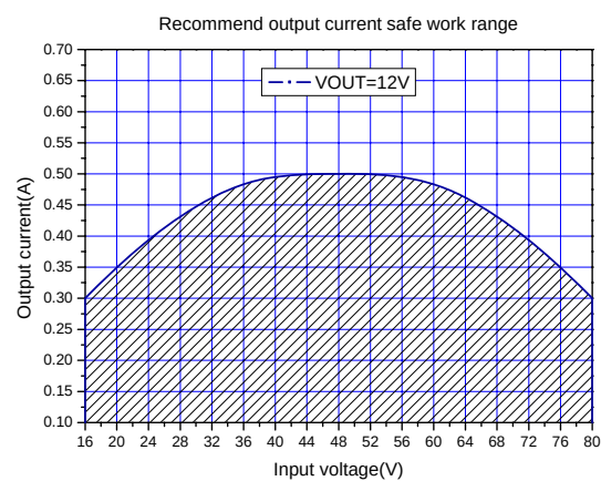
Figure6.Max output current(VOUT=12V)
