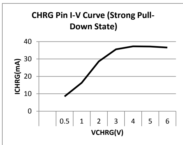
I-V curve
