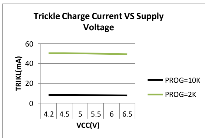
Relationship between trickle current and supply voltage
