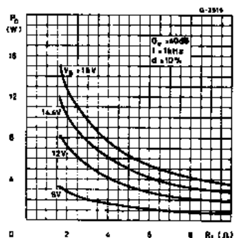
Figure 4. Output power vs. load resistance R_L
