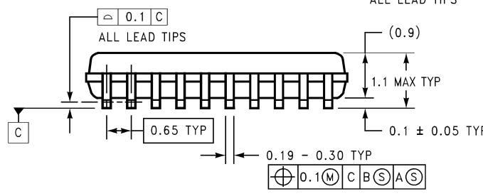
20-Lead Molded TSSOP, Exposed Pad, 6.5x4.4x0.9mm Order Number LM4863MTE NS Package Number MXA20A
