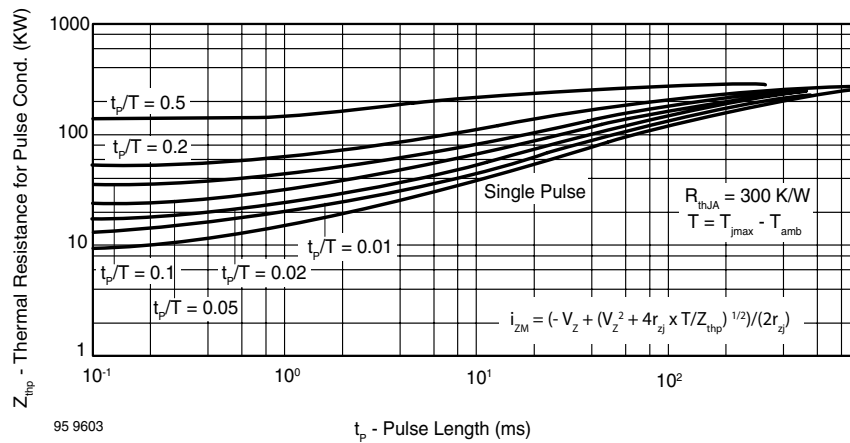
Figure 11. Thermal Response
