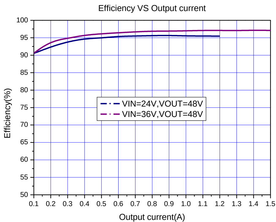
Figure16. XL6019 System Efficiency Curve (VIN=20~40V, VOUT=48V)
