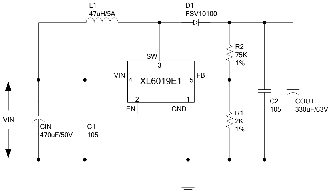
Figure19. XL6019 High Power Application Circuit (VIN=36V,VOUT=48V,IOUT=2.1A)
